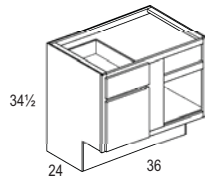
Base Corner - BC42 Stile: 6" Blind opening = 13 1/2"
