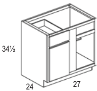
Base Corner - BC36 Stile: 6" Blind opening = 9"
