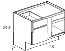
Base Corner - BC48 Stile: 6"
